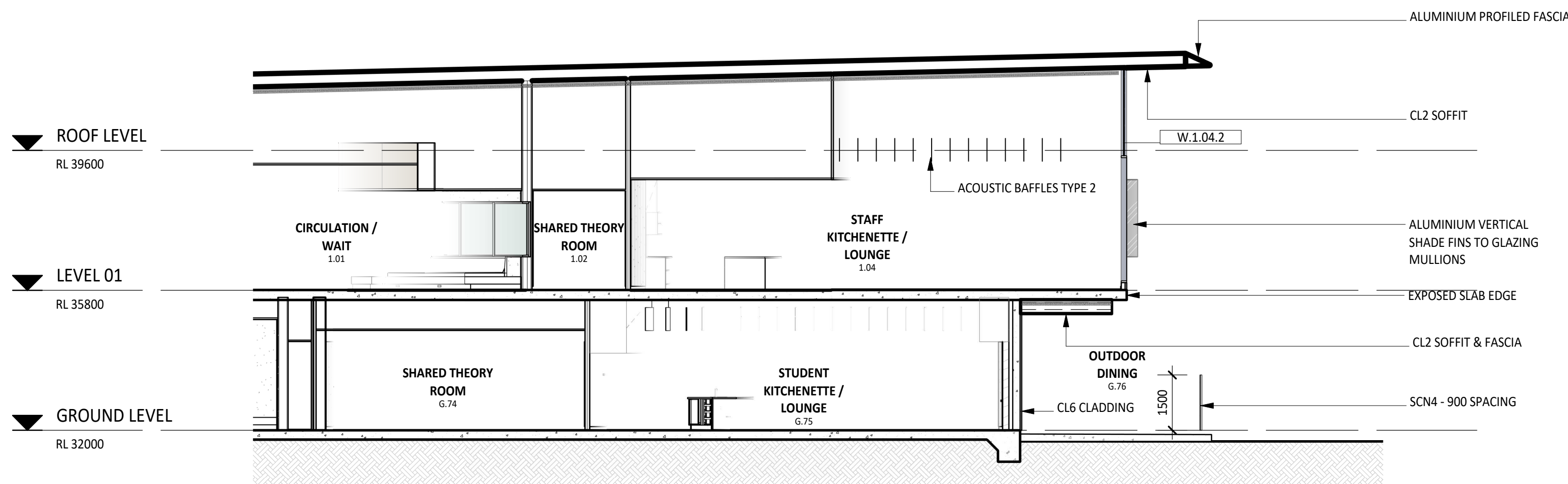
2 21-02 BUILDING SECTION - 11 1 : 100
