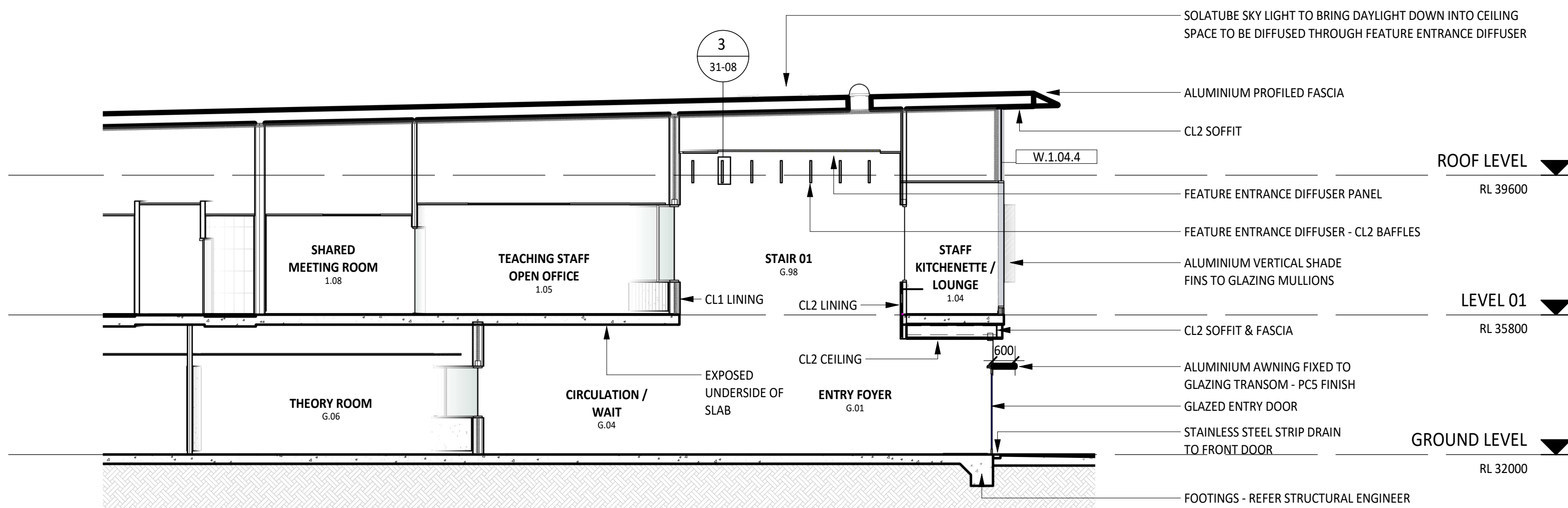
1 21-02 BUILDING SECTION - 10 1 : 100
